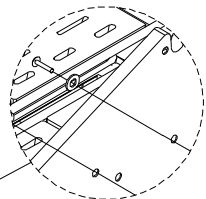
Phillips Head Screws 3/16"x3/8" with Plain Washer 3/16"
