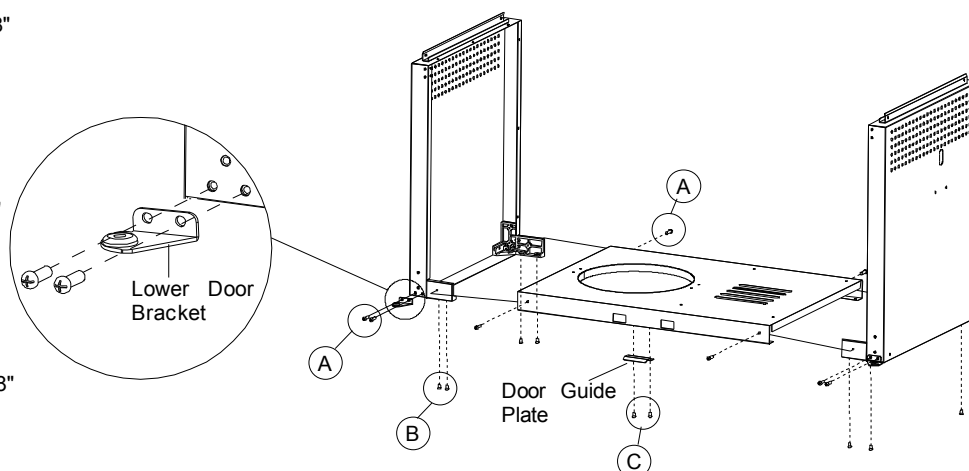
Pan Head Screw 1/4"x3/8" Qty. 8 Part # S182G0406A
