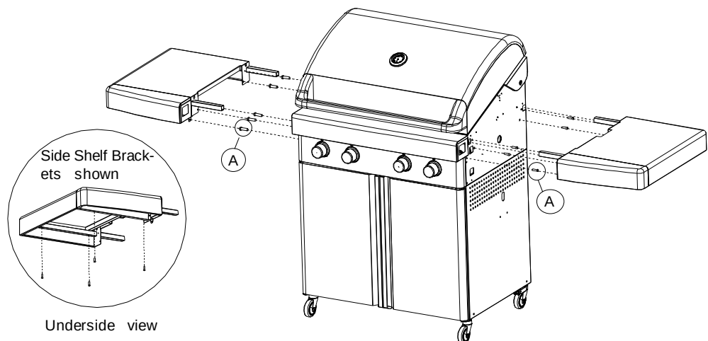
Pan Head Screw 3/16"x3/8" Qty. 8 Part # S182G0306A
