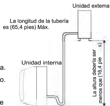
Outdoor unit is higher than indoor unit
