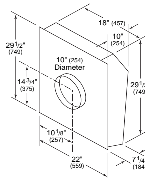
BLOWER-120REM
