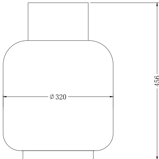
Propane tank: height = 456mm, diameter = 320mm
