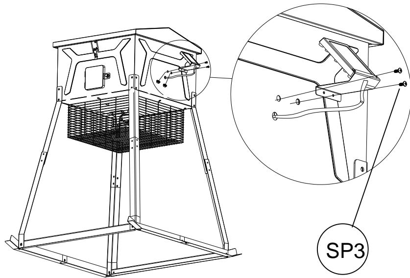
155060 Game Winner 6V Solar Panel Charger Assembly (not included)
