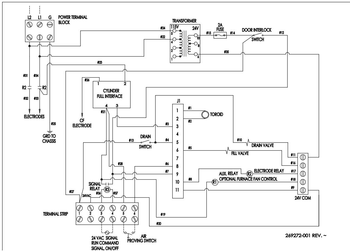
CFS22 Wiring Diagram
