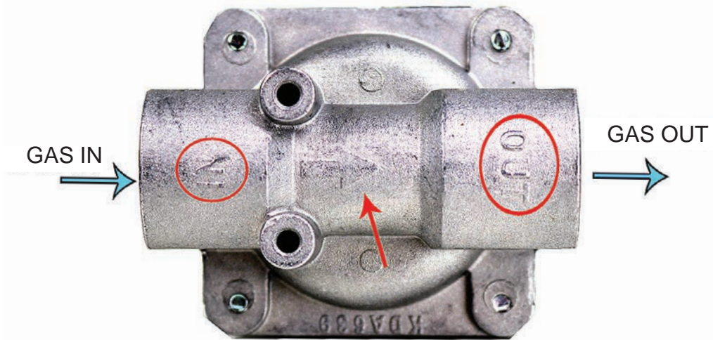
UNDERNEATH OF THE REGULATOR
