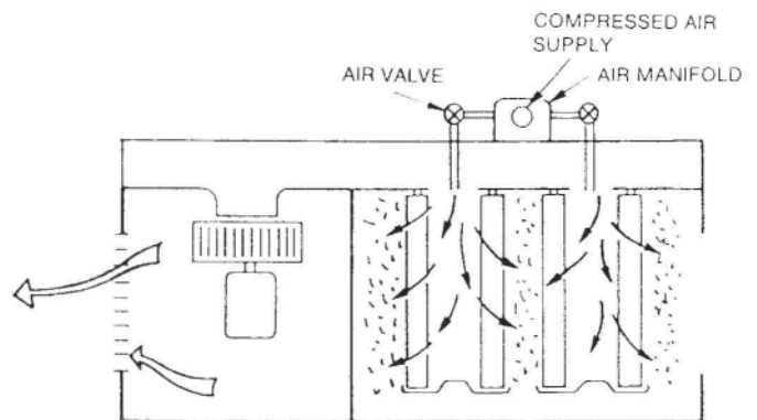
AIR FLOW, PURGING/CLEANING CYCLE (TOP VIEW)
