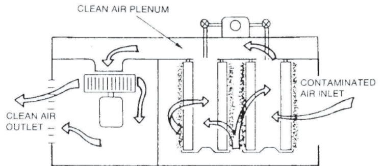
AIR FLOW, NORMAL OPERATION (TOP VIEW)
