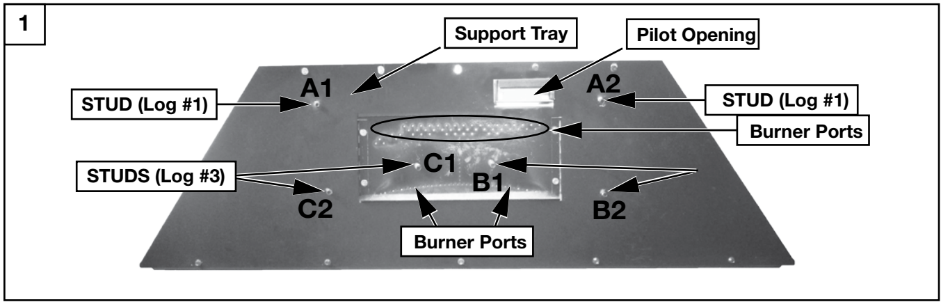
Burner Overview
