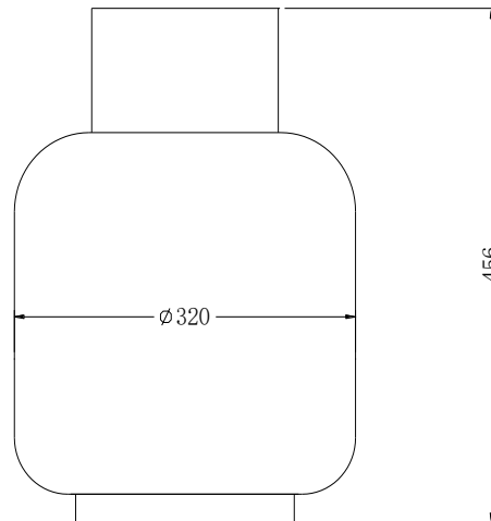
Propane tank: height = 456mm, diameter = 320mm
