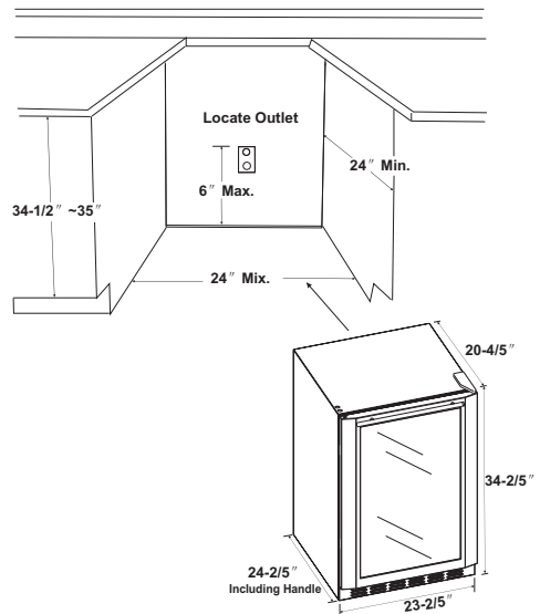
Figure A – The cutout depth must be 24"
