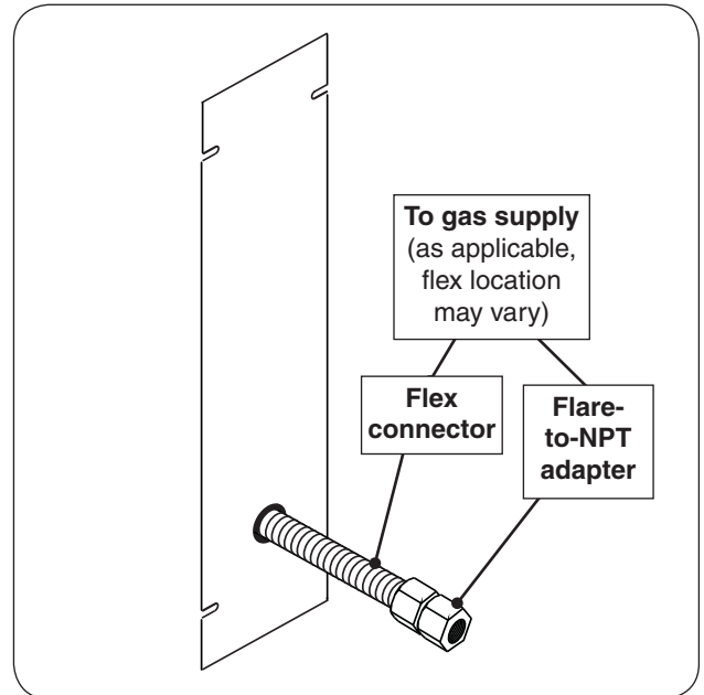
Fig. 18-1 Connect gas and secure plate
