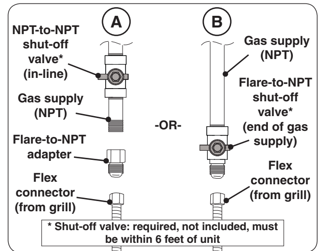
Fig. 18-2 Connecting to a gas line
