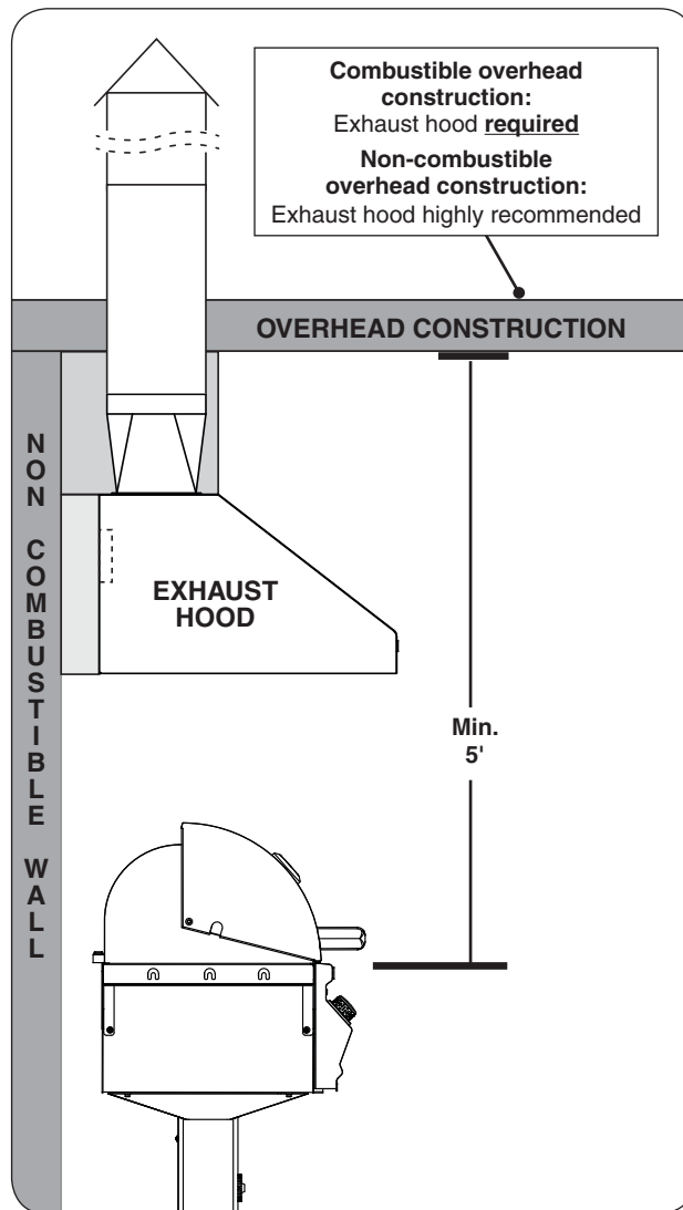
Fig. 8-1 Overhead requirements
