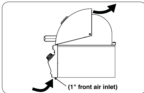
Fig. 10-1 Airflow diagram
