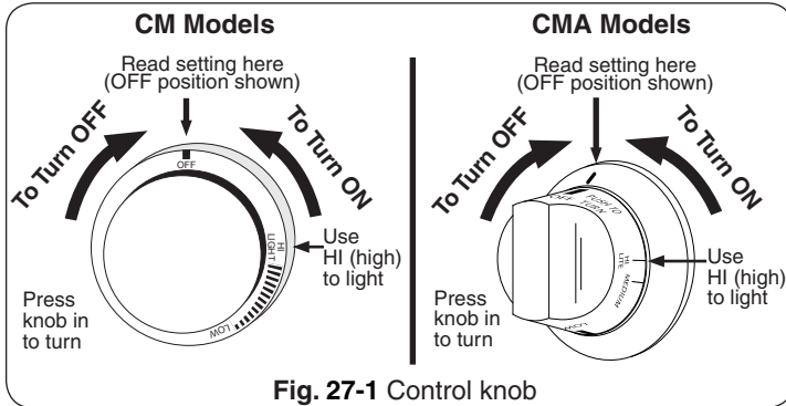
Fig. 27-1 Control knob
