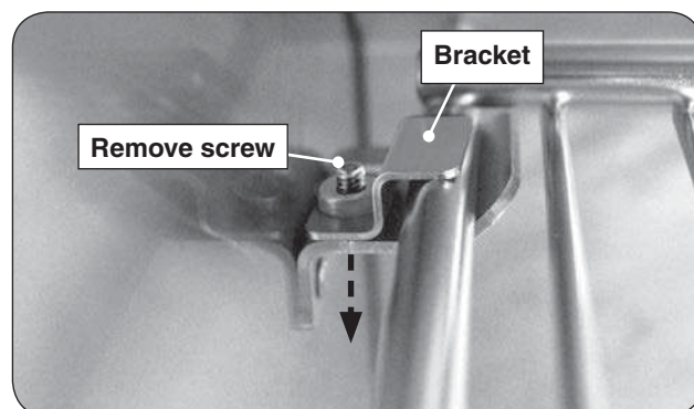
Fig. 33-3 Warming rack locking bracket removal
