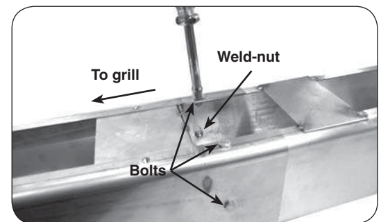
Fig. 20-2 Fasten extension to post
