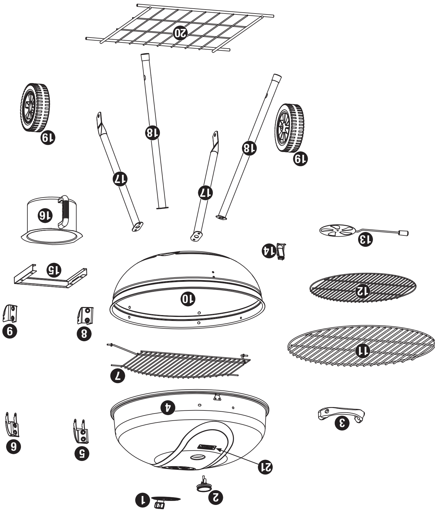
Expanded View
