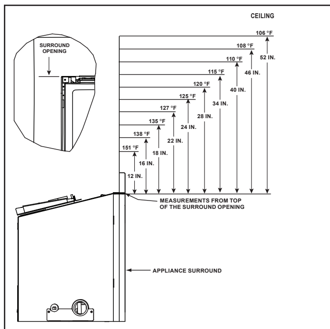
Figure 3.3 Good Faith Wall Surface Temperatures Above Appliance
