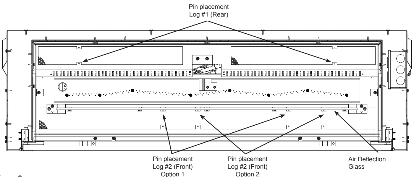
Figure 2 – Alternative Log Placement
