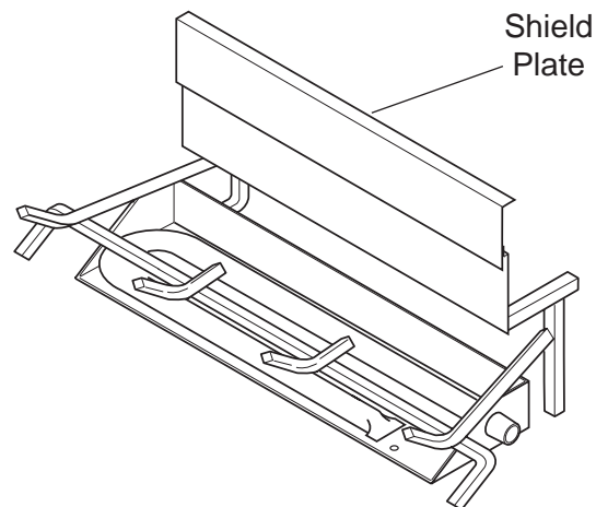
Figure 67 - Sliding Shield Plate Down Back of Burner Pan
