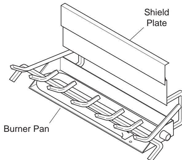
Figure 34 - Sliding Shield Plate Down Back of Burner Pan
