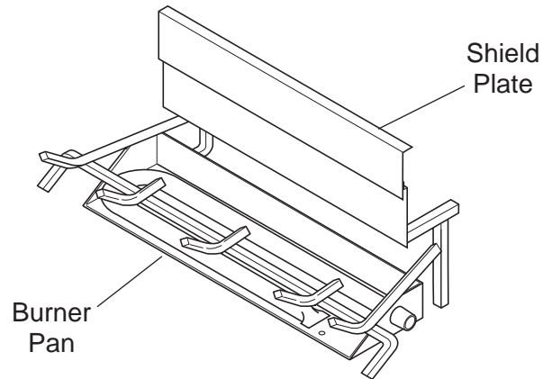
Figure 18 - Sliding Shield Plate Down Back of Burner Pan
