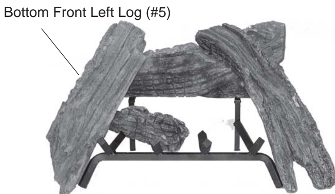
Figure 71 - Installing Bottom Front Left Log (#5)
