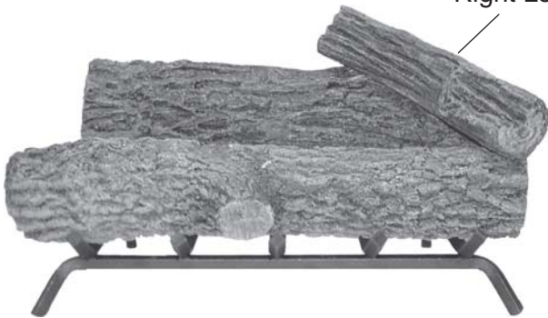
Figure 54 - Positioning Right Log (#3)
