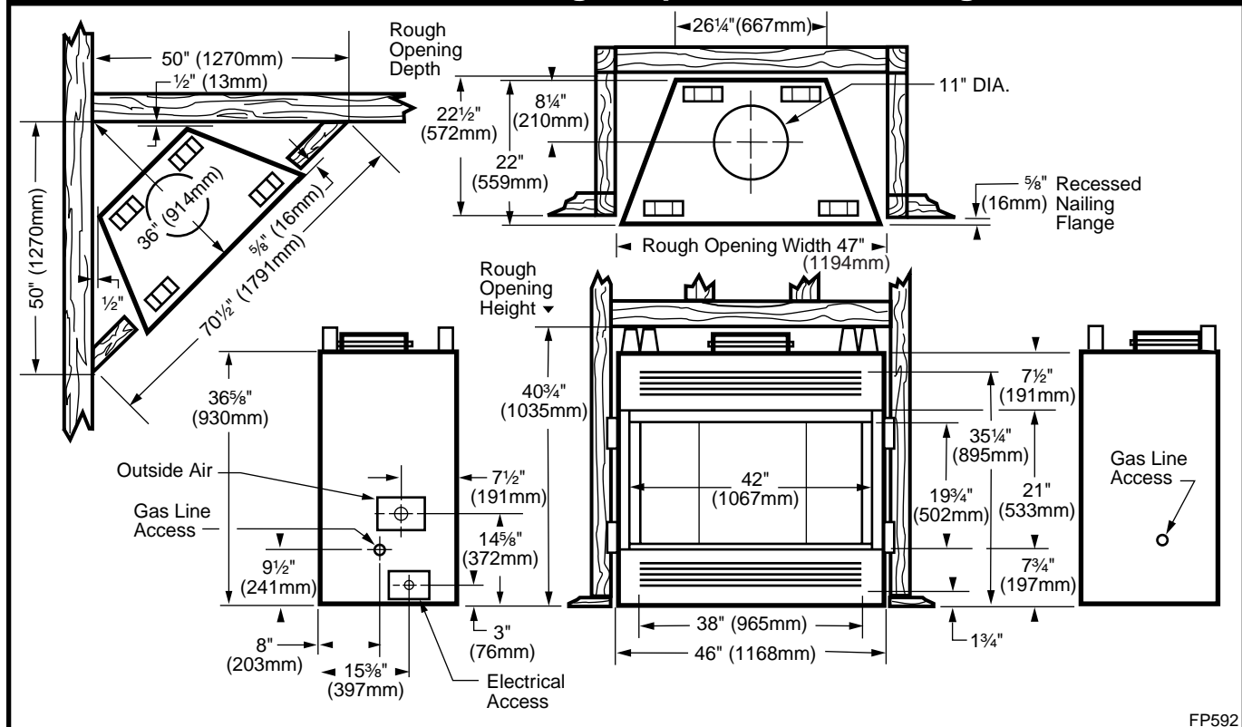
Fig. 4 SC42 Series specifications and framing.
