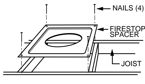
Fig. 18 Installing firestop spacer.
