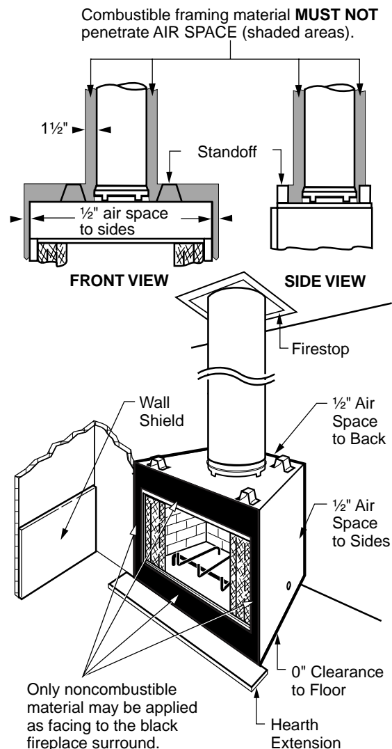
Fig. 20 Minimum clearances to combustibles.
