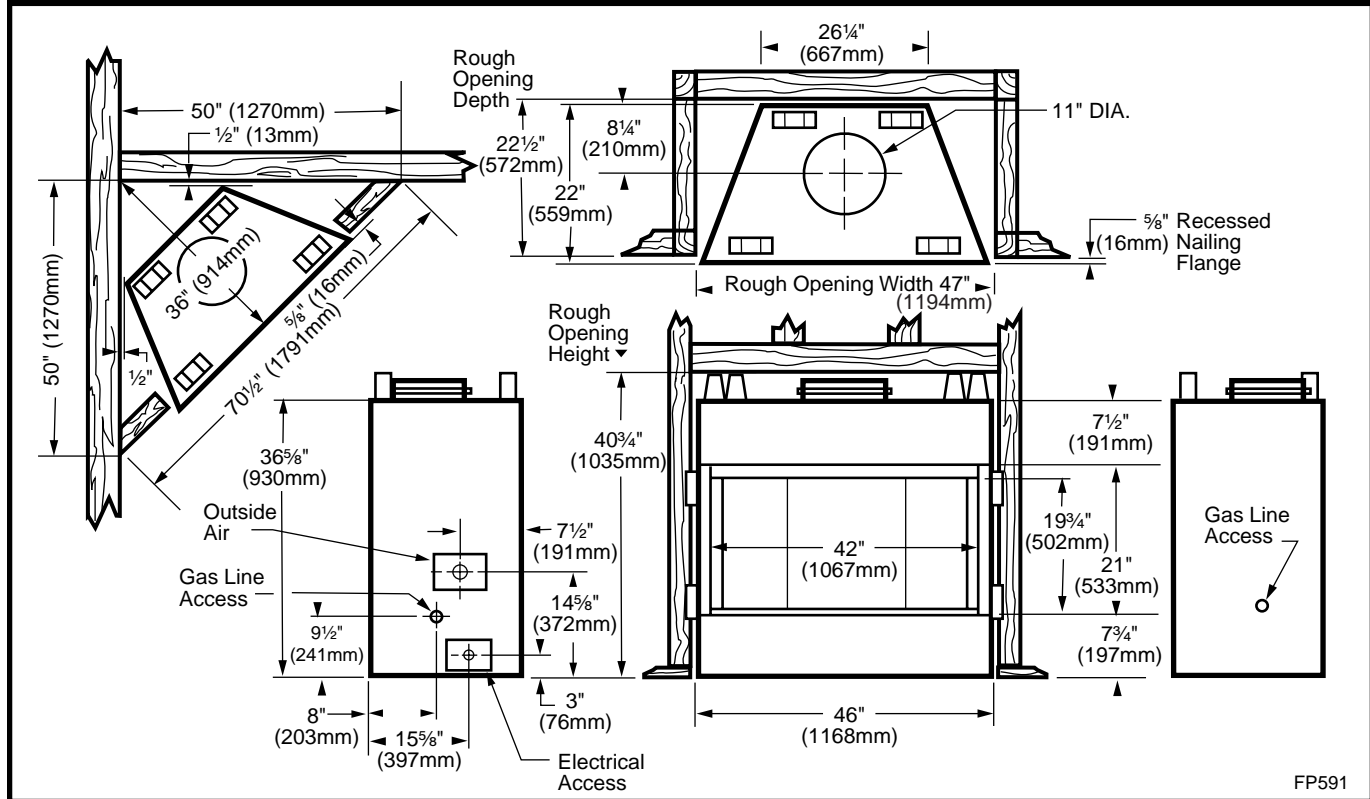
Fig. 3 SR42 Series specifications and framing.
