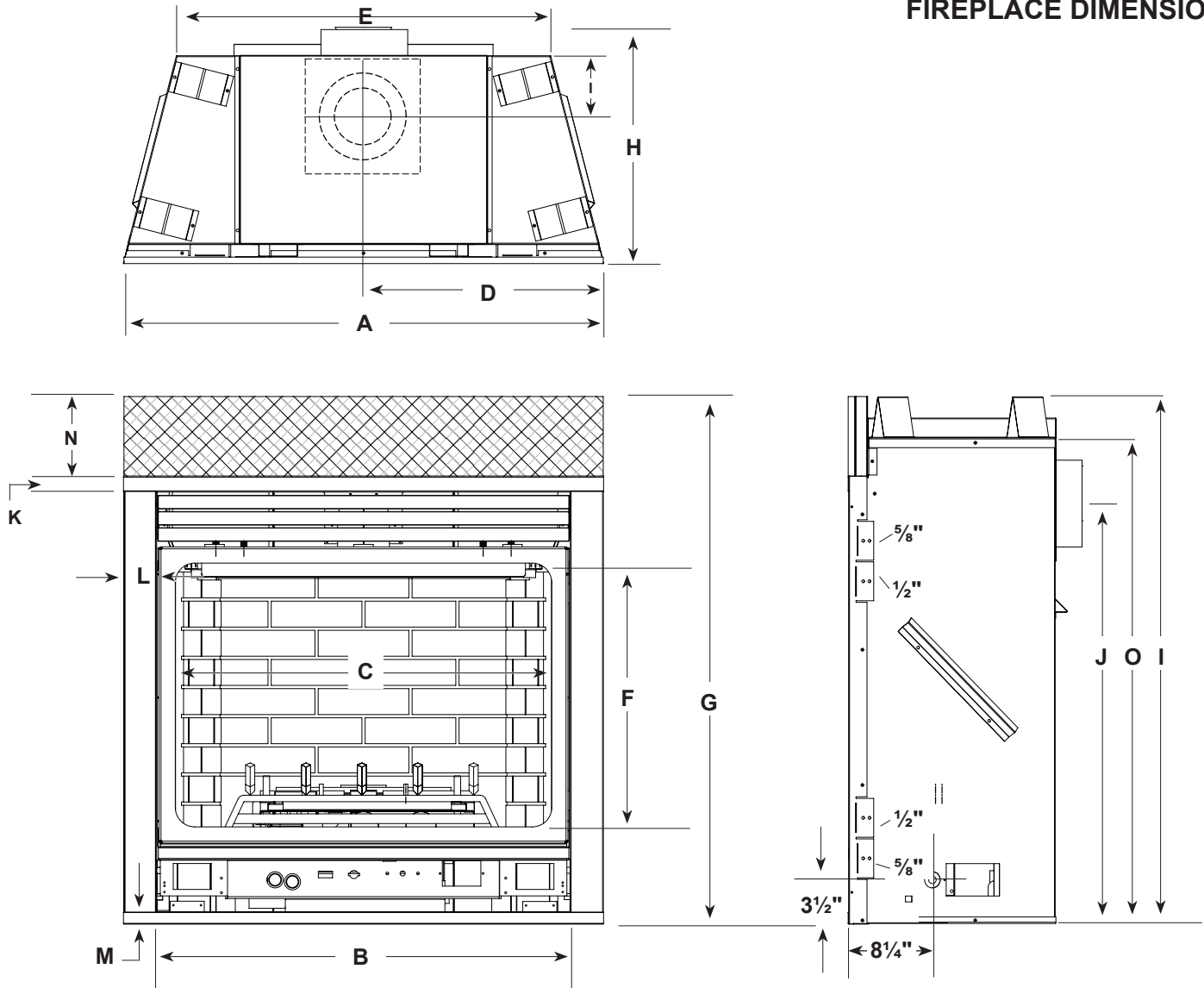
Figure 3 - Fireplace Dimensions
