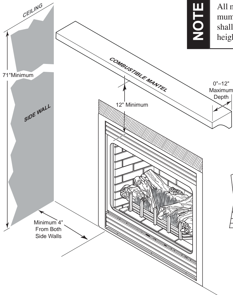
Figure 5 - Clearances
