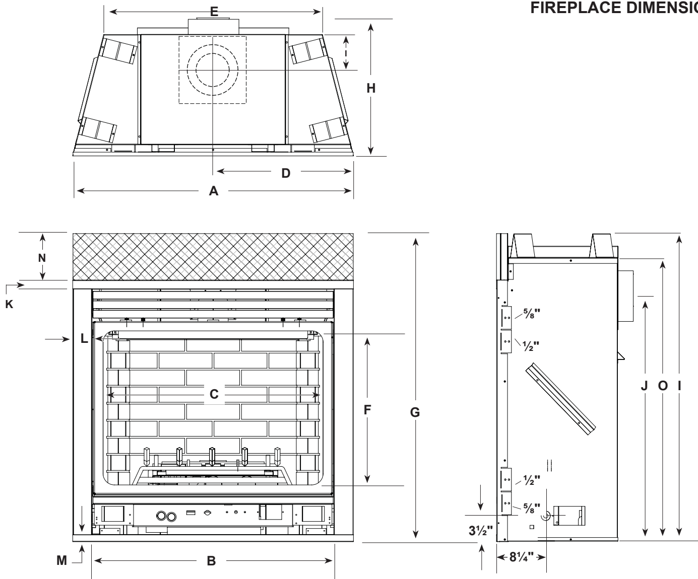
Figure 3 - Fireplace Dimensions
