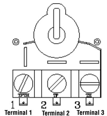
Gas Valve Wiring Terminals
