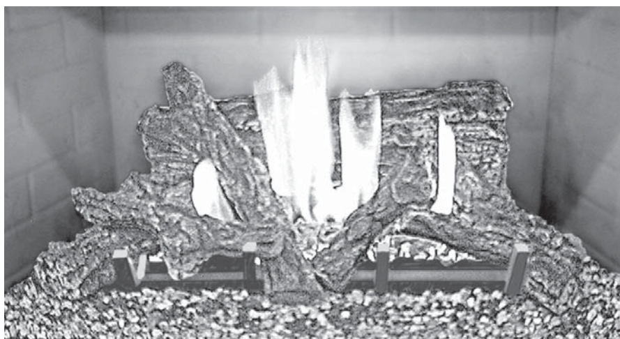
Figure 11 Burner Flame Appearance - Model MPB-3530
