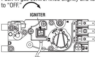
HONEYWELL MILLIVOLT GAS VALVE
