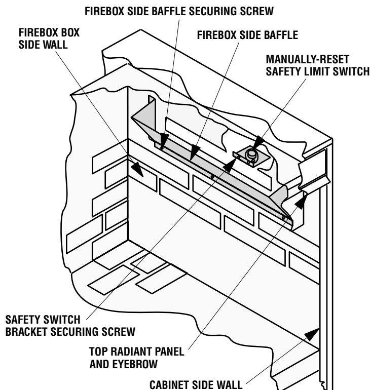
SAFETY SWITCH LOCATION (EBVCL SHOWN) EBBST and EBVPF Safety Switch Location Also as Shown; EBVCR Location on Left End of Fireplace.
