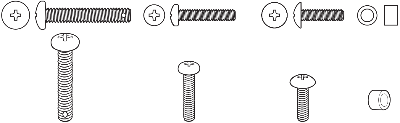
PHILLIPS PAN HEAD SCREW, SS, 1/4-20 X 1-1/2 B101649 (1)
