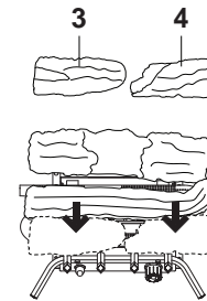
Fig. 21 - Installing Log #3 & Log #4
