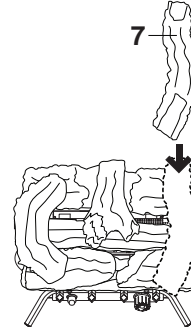
Fig. 24 - Installing Log #7
