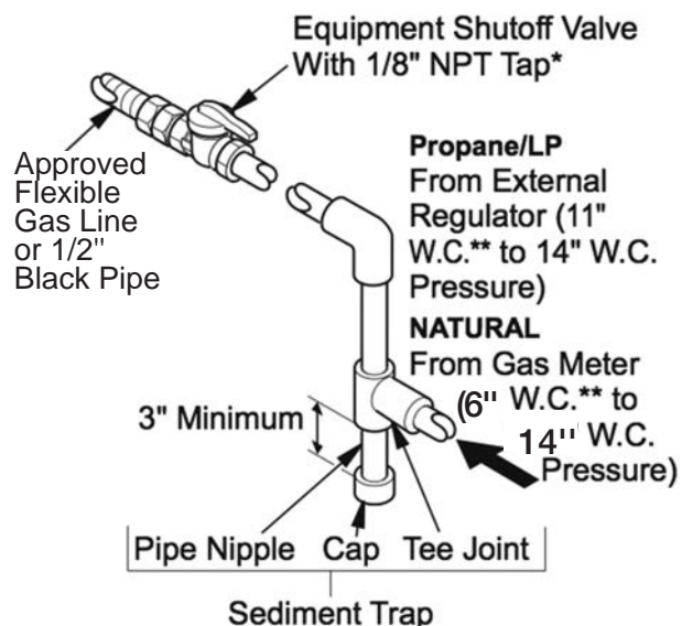
Fig. 15 - Gas Connection
