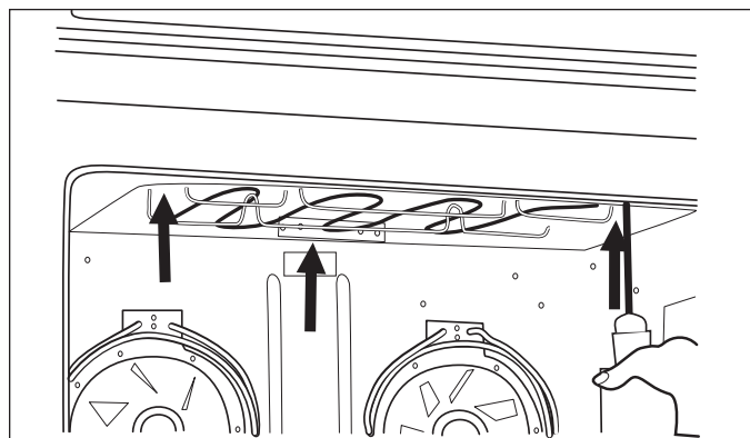
Figure 4-32. Broil Element Removal.
