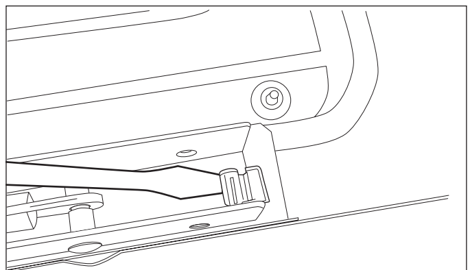
Figure 4-43. Raising Tab for Hinge Removal.
