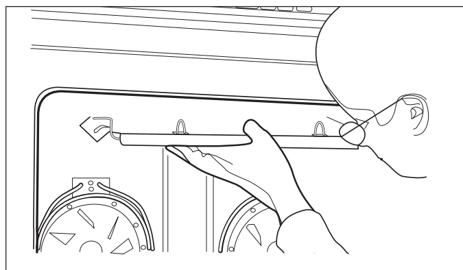
Figure 4-33. Broil Element Removal.
