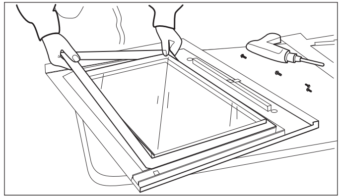
Figure 4-40. Removing Inner Heat Shield.
