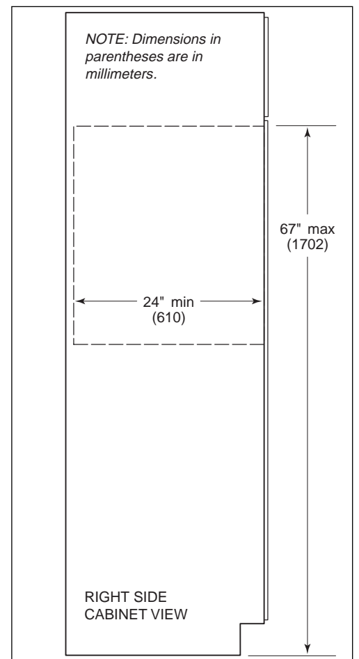
Figure 2-8. Side View
