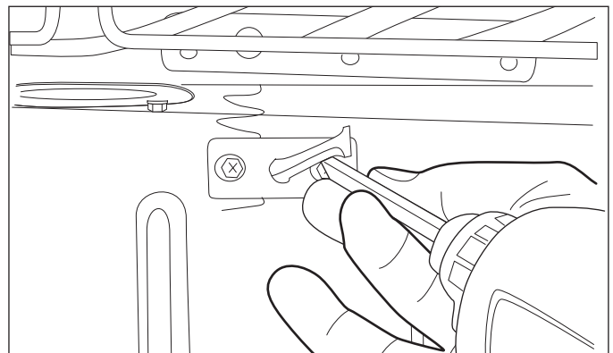
Figure 4-29. Temperature Sensor Removal.
