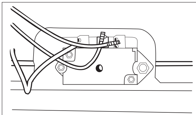
Figure 4-35. Bake Stone Receptacle Removal.
