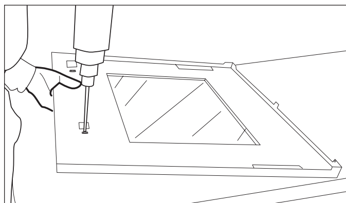
Figure 4-38. Outer Door Skin Removal.
