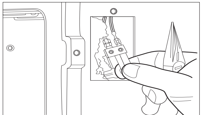
Figure 4-28. Probe Switch Removal.
