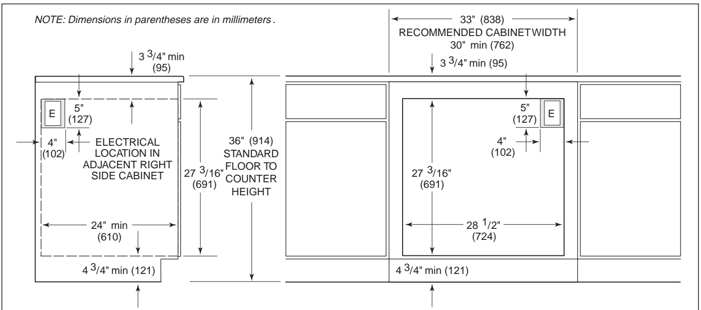
Figure 2-6. Undercounter Cutout Dimensions and Electrical Placement
