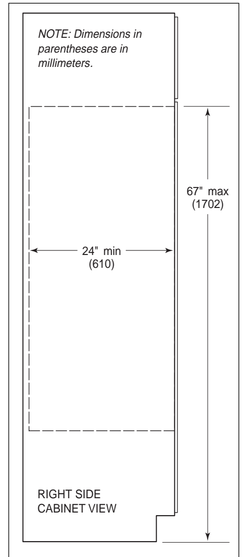
Figure 2-13. Side View
