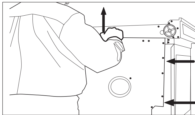
Figure 4-50. Enclosure Removal.
