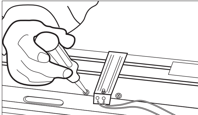
Figure 4-7. Switch Actuator Removal.
