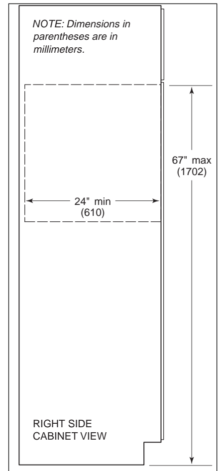
Figure 2-11. Side View
