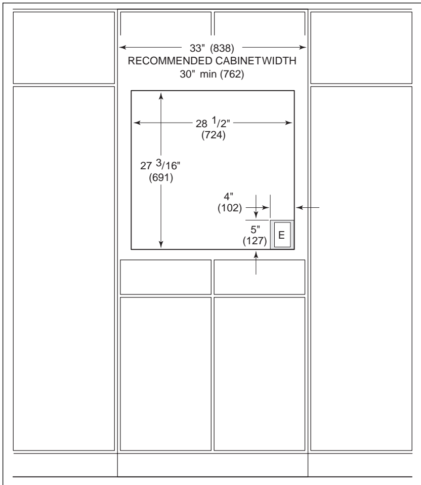
Figure 2-7. Front Cutout Dimensions and Electrical Placement
