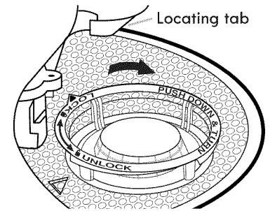
To replace Upper Filter Assembly
